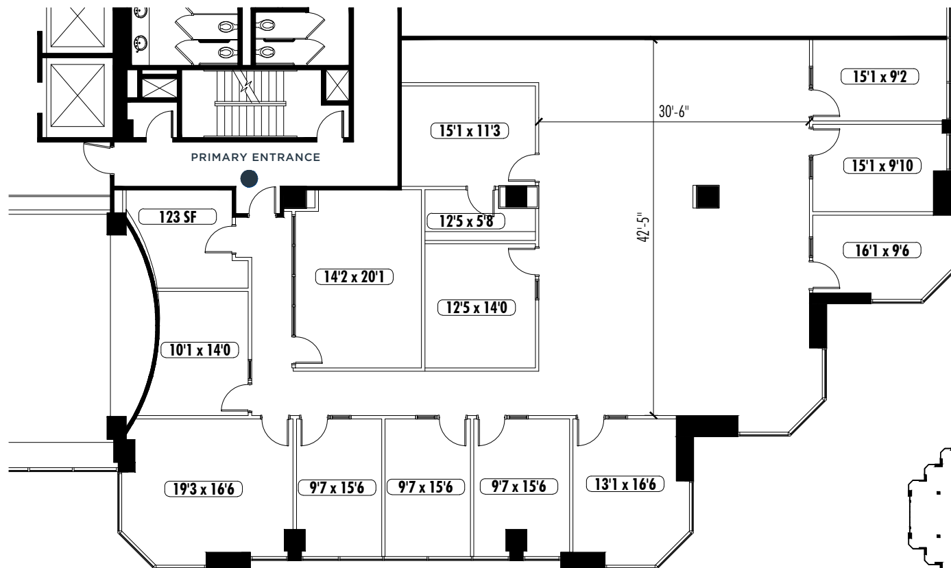
KEY PLAN
